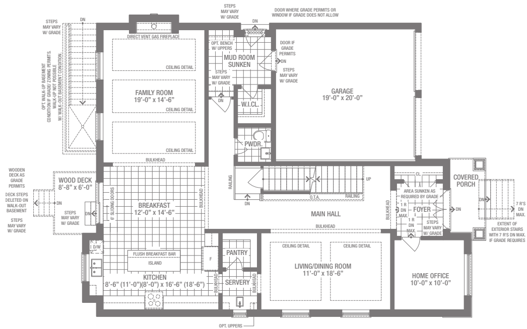
GROUND LEVEL
