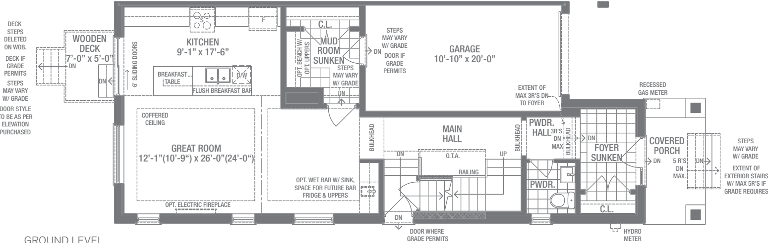
GROUND LEVEL
