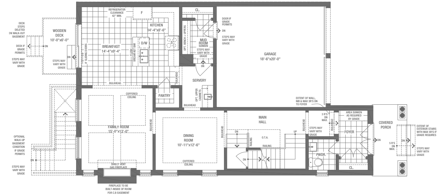
GROUND FLOOR
